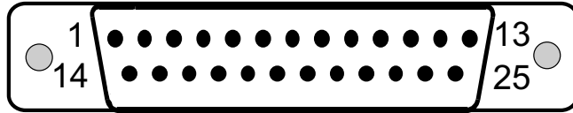
25-way D-type male connector at the back of the indicator
